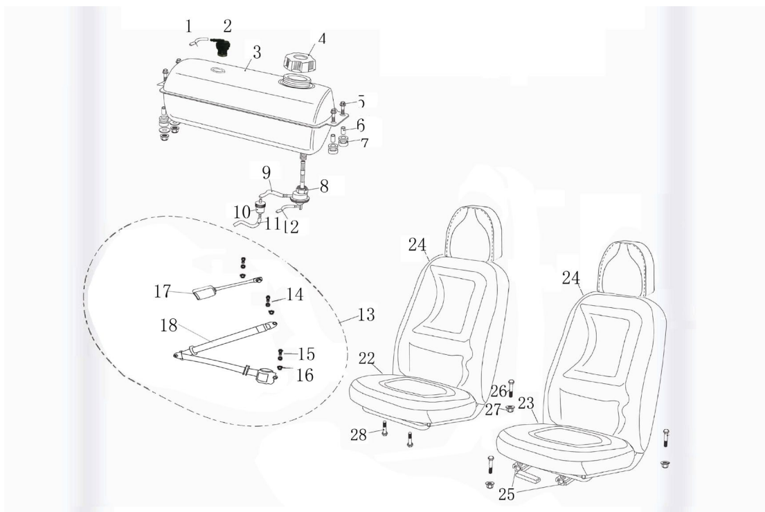
Fig 20: TANK/SEAT/SEATBELT
