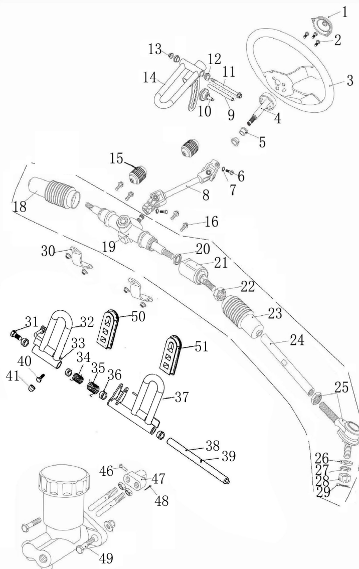
Fig 18: STEERING SHAFT ASSY
